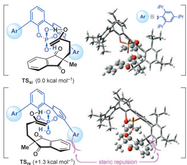
Figure 1. 3D structures and schematic representation of models of TS re and TS si calculated by ONIOM (B3LYP/−31G*:HF/3-21G).
