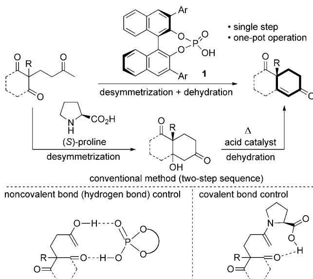
Scheme 1. Synthetic strategy for the preparation of chiral cyclohexenones.
